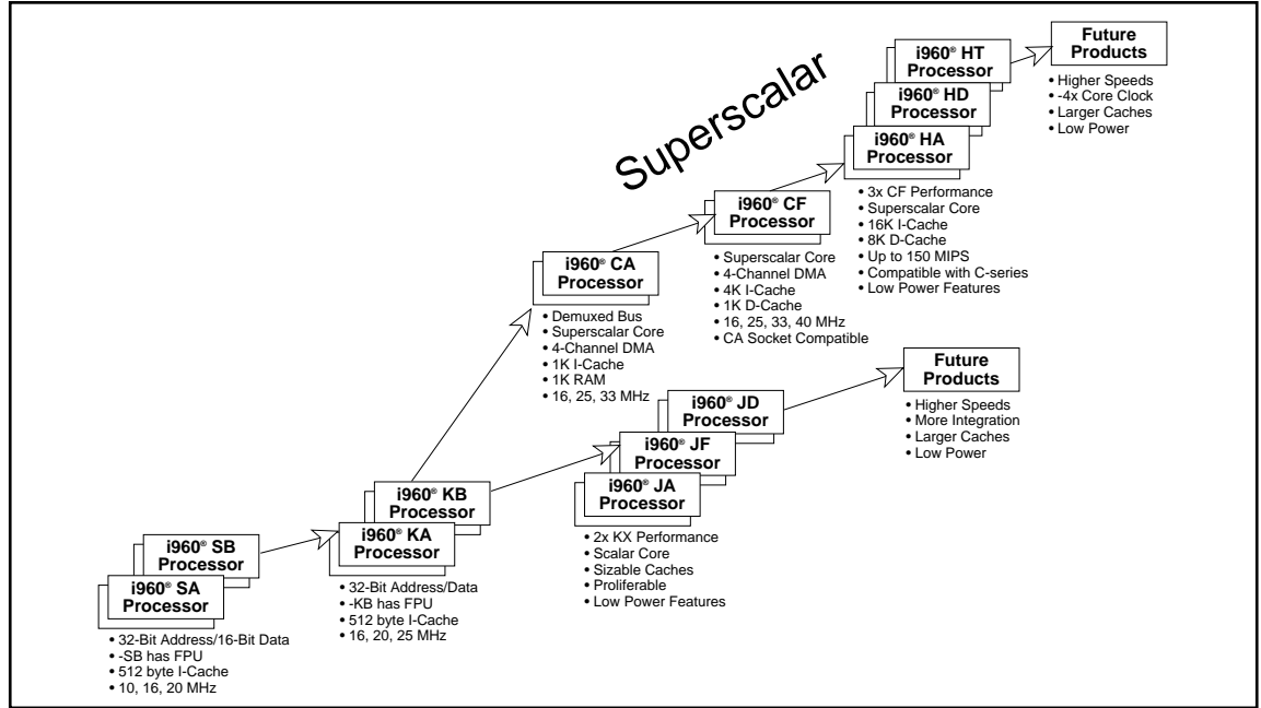
Room to Grow: i960 ® Microprocessor Roadmap
