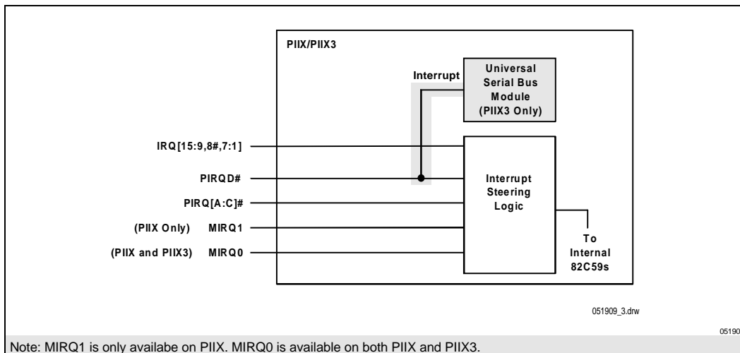
Figure 8. Interrupt Steering
