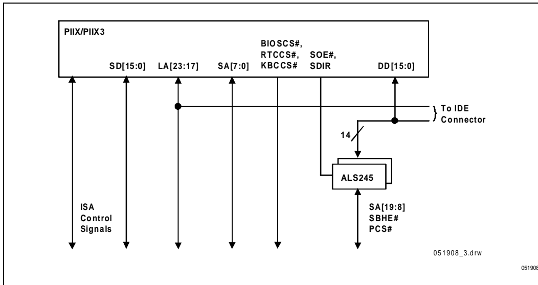
Figure 1. ISA Interface
