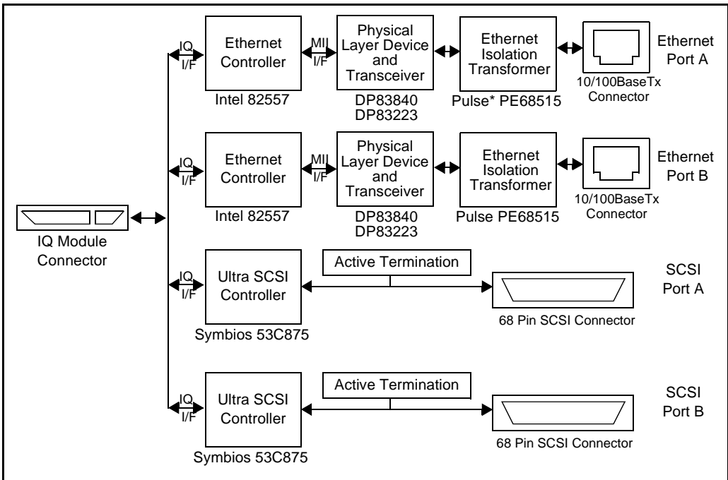
Figure 3-1. SCSI/Ethernet IQ Module Block Diagram
