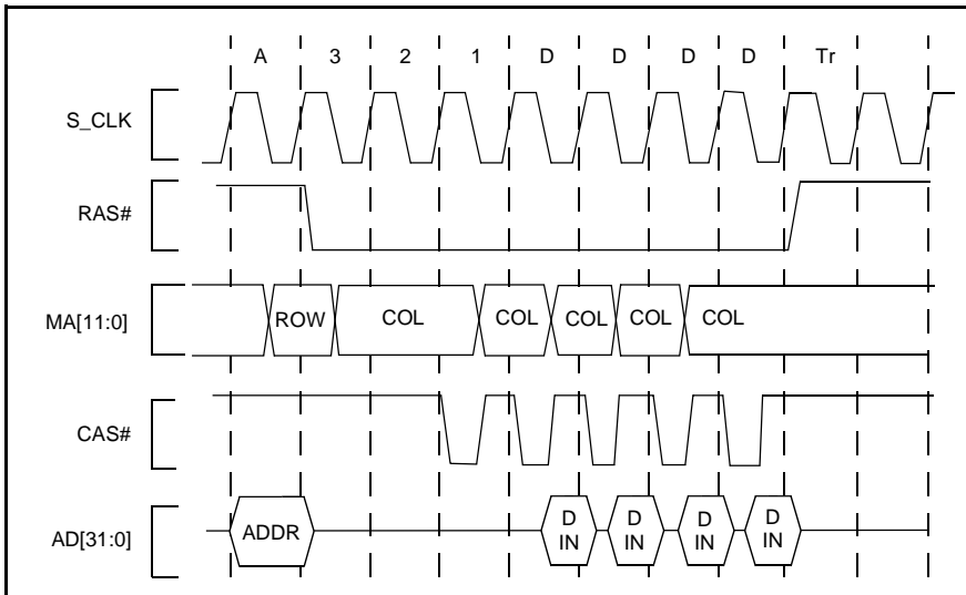
Figure 22. BEDO DRAM, Read Cycle
