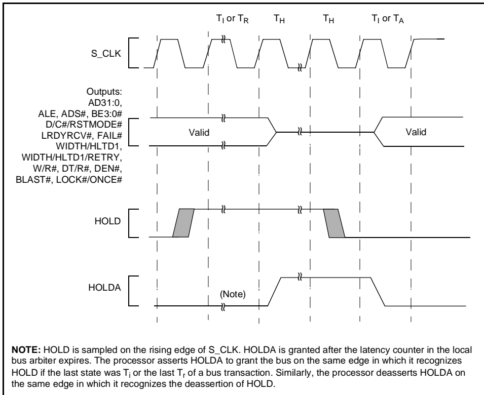
Figure 32. HOLD/HOLDA Waveform For Bus Arbitration
