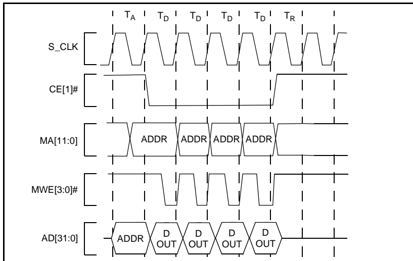
Figure 25. 32-Bit Bus, SRAM Write Accesses with 0 Wait States
