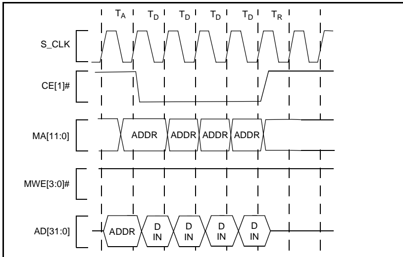
Figure 24. 32-Bit Bus, SRAM Read Accesses with 0 Wait States
