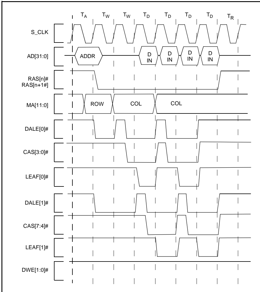
Figure 18. FPM DRAM System Read Access, Interleaved, 2,0,0,0 Wait States
