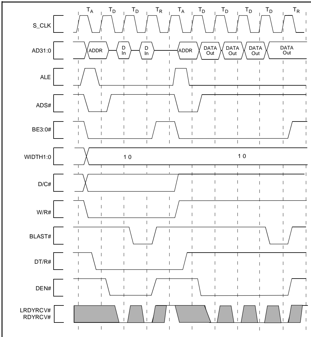
Figure 27. Burst Read and Write Transactions without Wait States, 32-Bit 80960 Local Bus
