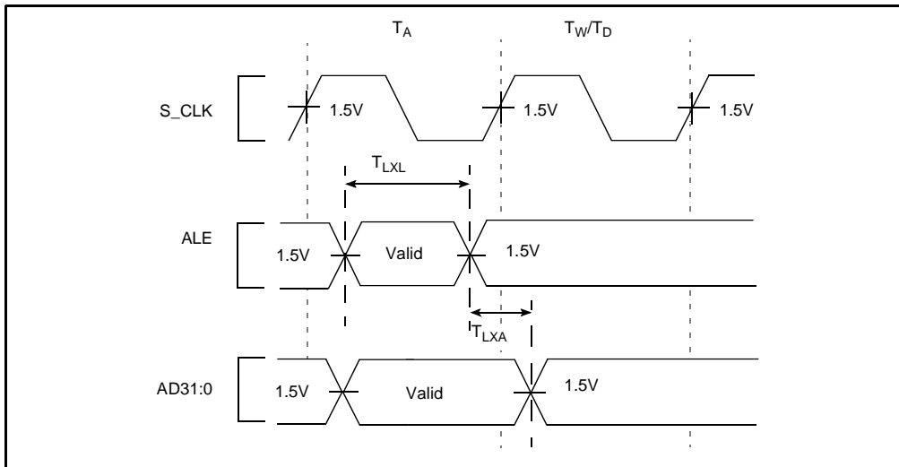
Figure 13. T_{LXL} and T_{LXA} Relative Timings Waveform
