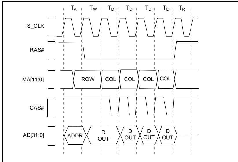
Figure 21. EDO DRAM, Write Cycle
