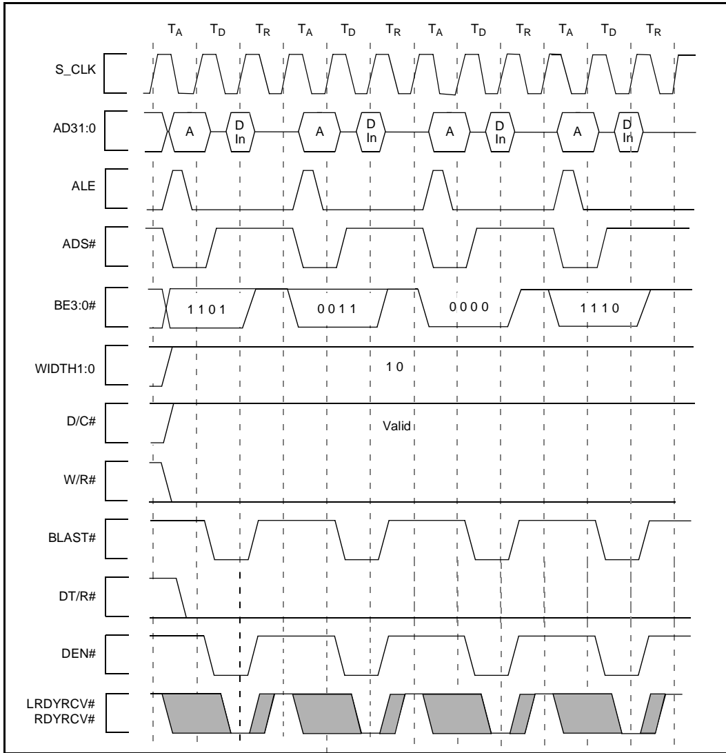
Figure 31. Bus Transactions Generated by Double Word Read Bus Request, Misaligned One Byte From Quad Word Boundary, 32-Bit 80960 Local Bus, Little Endian
