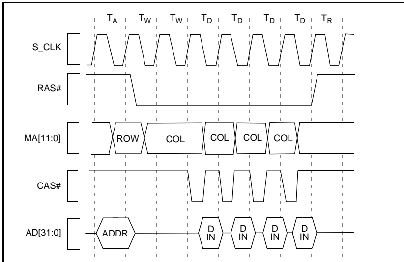
Figure 20. EDO DRAM, Read Cycle
