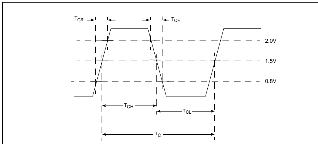
Figure 9. S_CLK, TCLK Waveform
