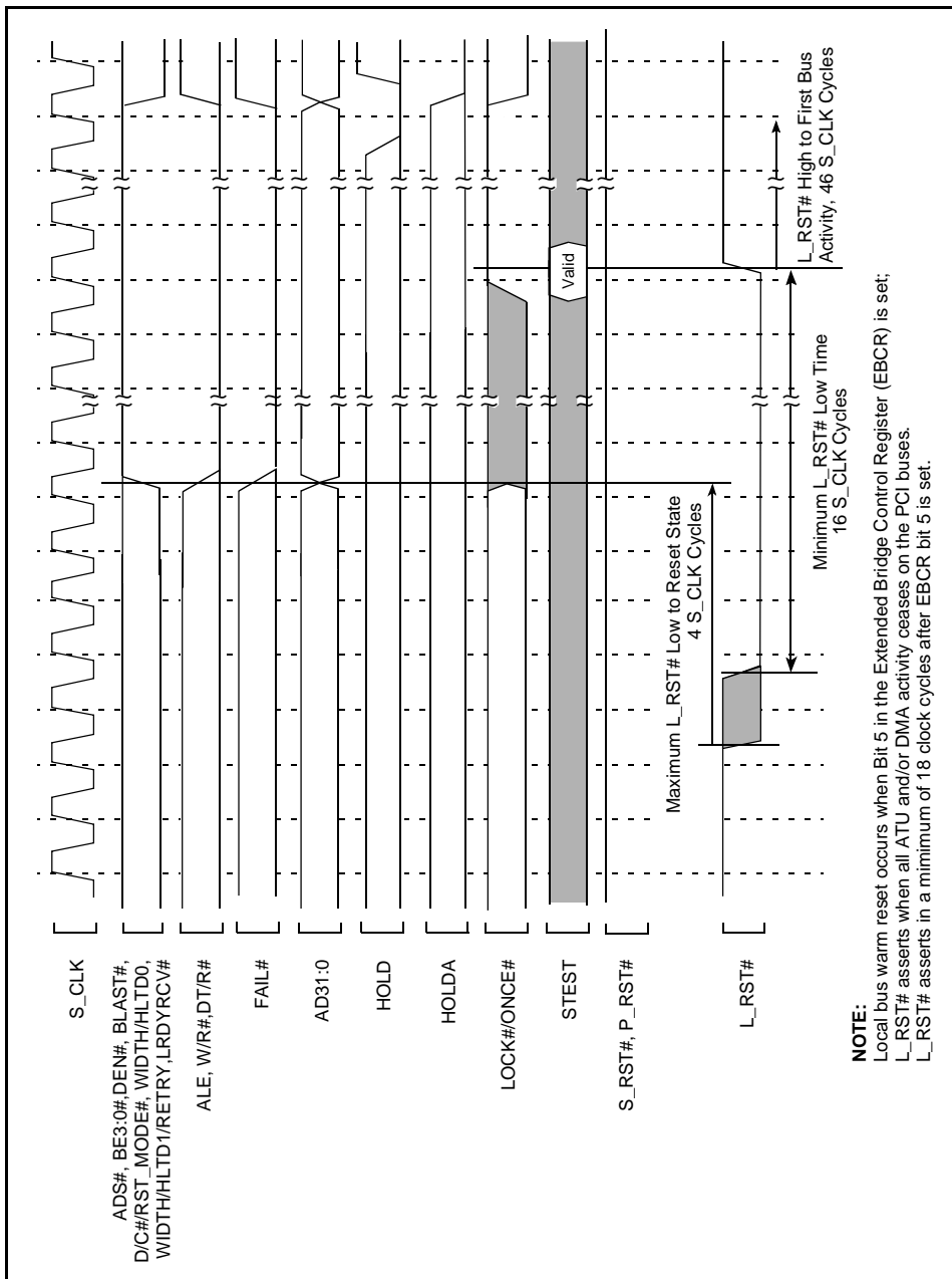
Figure 34. 80960 Local Bus Warm Reset Waveform
