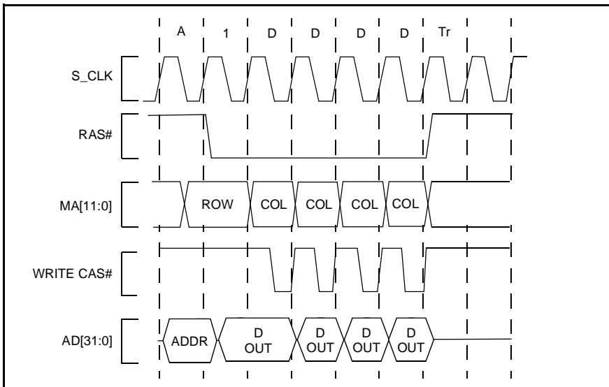
Figure 23. BEDO DRAM, Write Cycle
