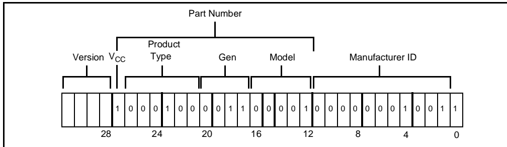
Figure 35. 80960Rx Device ID Register (DEVICEID)
