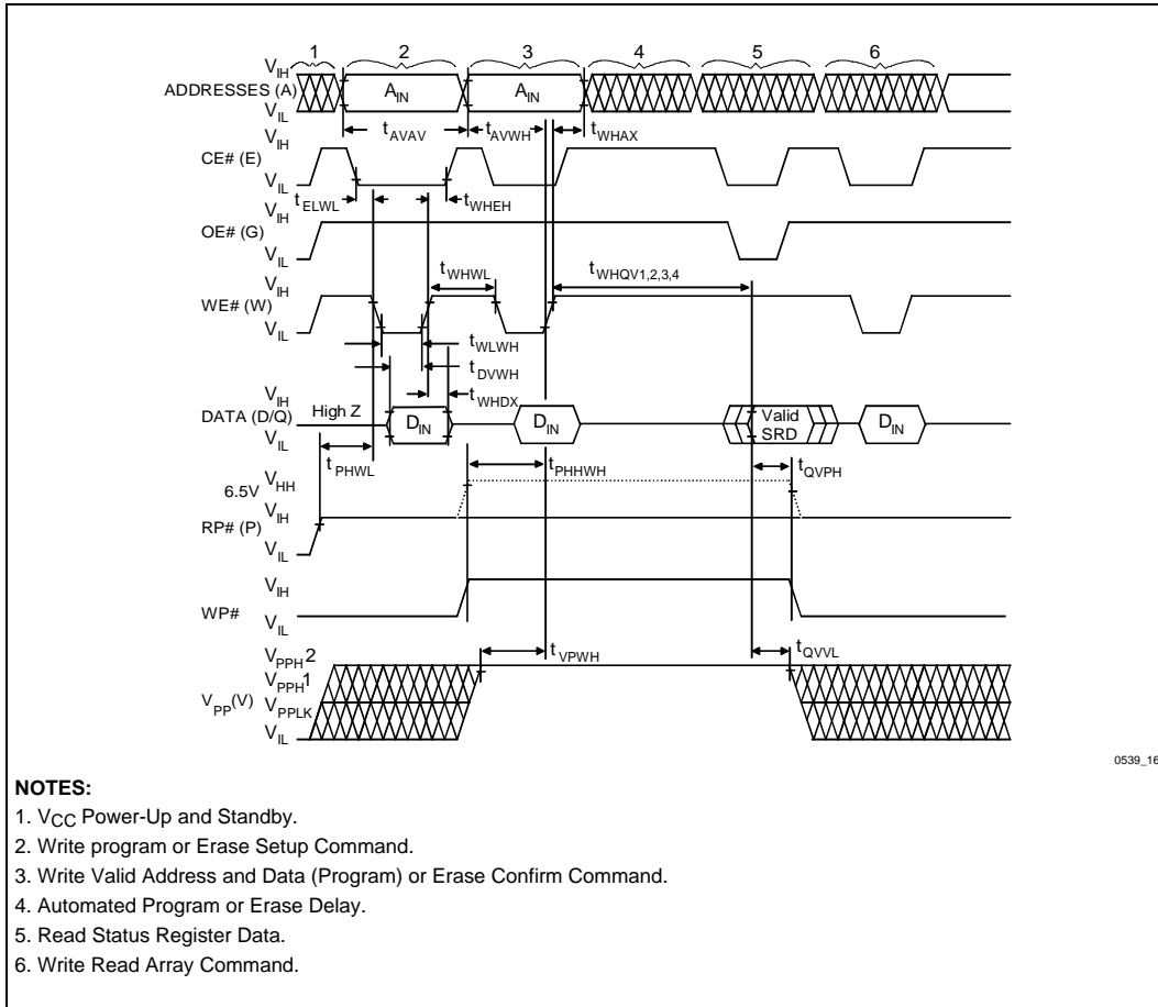
Figure 14. AC Waveforms for Write Operations (WE#-Controlled Writes)
