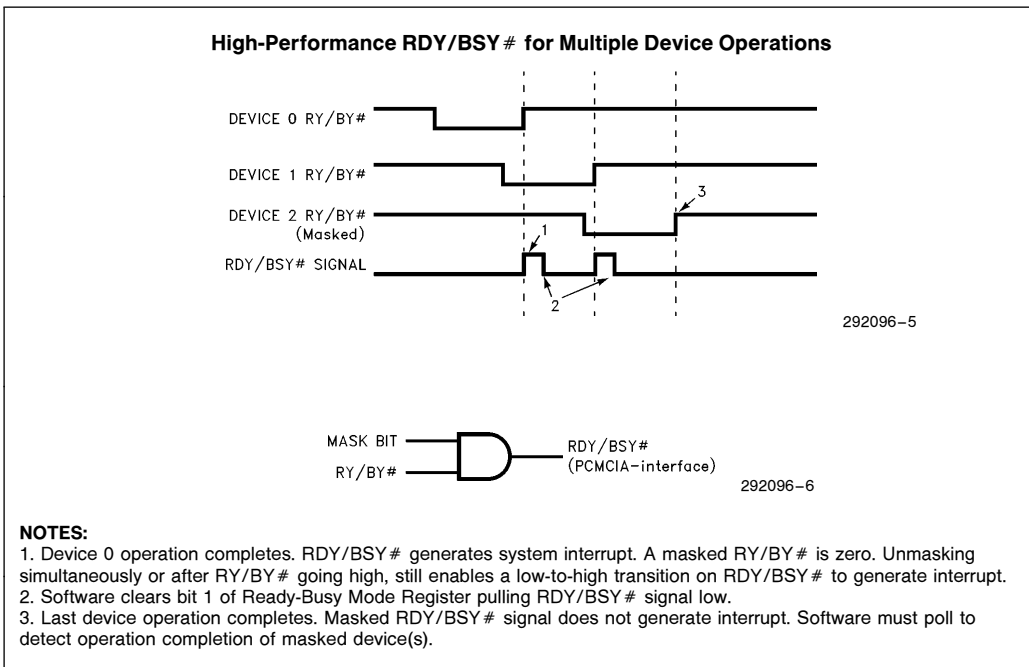
Figure 13. High-Performance Mode Catches Each Device Going Ready
