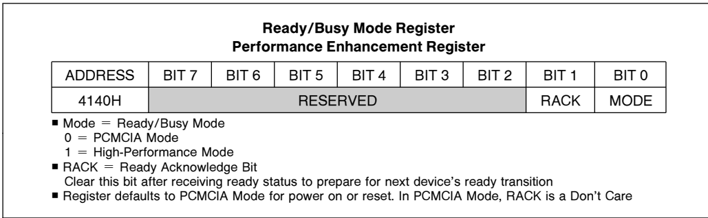
Figure 14. To Prevent Accidental Ready Transitions, a Three Step Sequence must be Followed to Enter High-Performance Mode
