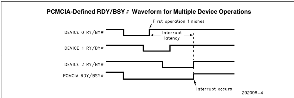
Figure 12. PCMCIA-Defined RDY/BSY Waveform for Multiple-Device Operations
