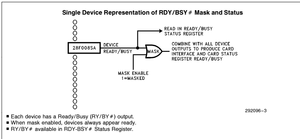
Figure 11. The Ready-Busy Mask is Very Useful for Write Optimization
